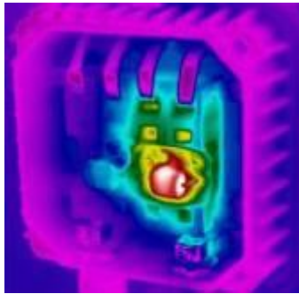
Figure 35 - Surchauffe d'une diode bypass
